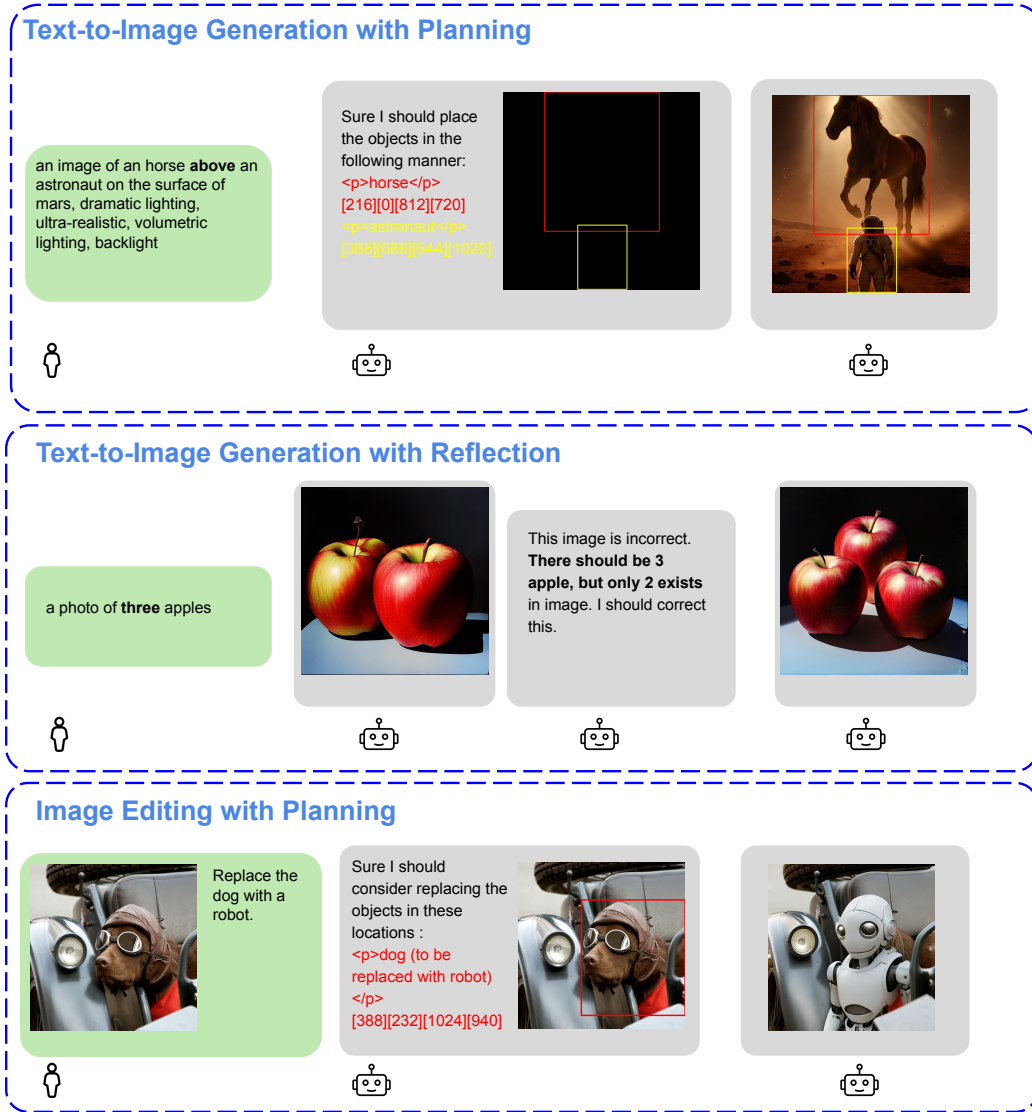
Figure 11: Interleaved Generation with Planning and Reflection. We provide visual examples of interleaved generation, including text-to-image generation with planning (Top), text-to-image generation with reflection (Middle), and image editing with planning (Bottom). We always enable planning during the reflection process. The layout traces is omitted in the middle figure for clarity and better presentation.
