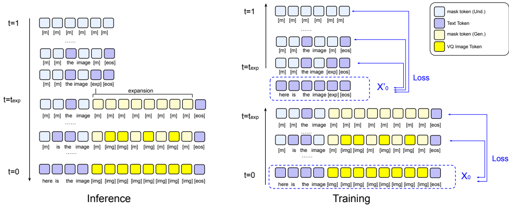
Figure 7: Training and inference with modality-aware masking. We visualize the sampling process with modality-aware masking on the left and the training process on the right. During the training, the loss is applied on either X_0 or X'_0 depending on the value of t with respect to t_{\text{exp}} .
